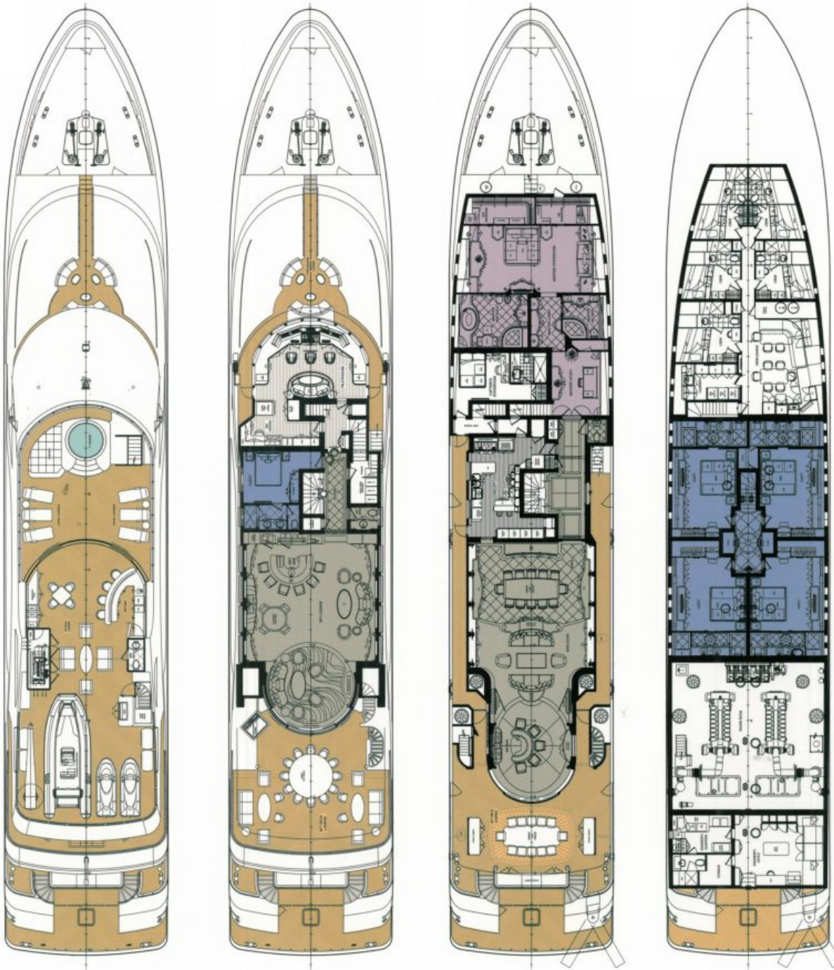
LADY SARA, 187' (56.96m) Trinity Motoryacht, 2012
