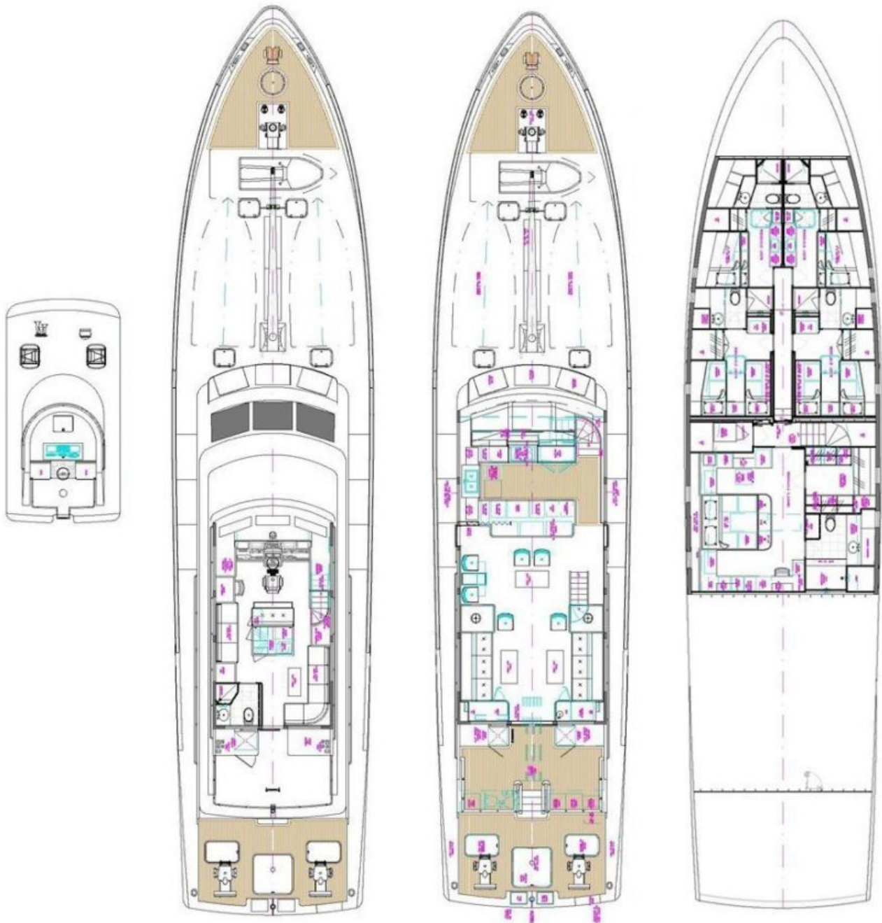
DREAM CATCHER, 108' (32.92m) Burger Sport Fisherman, 2001/2014
